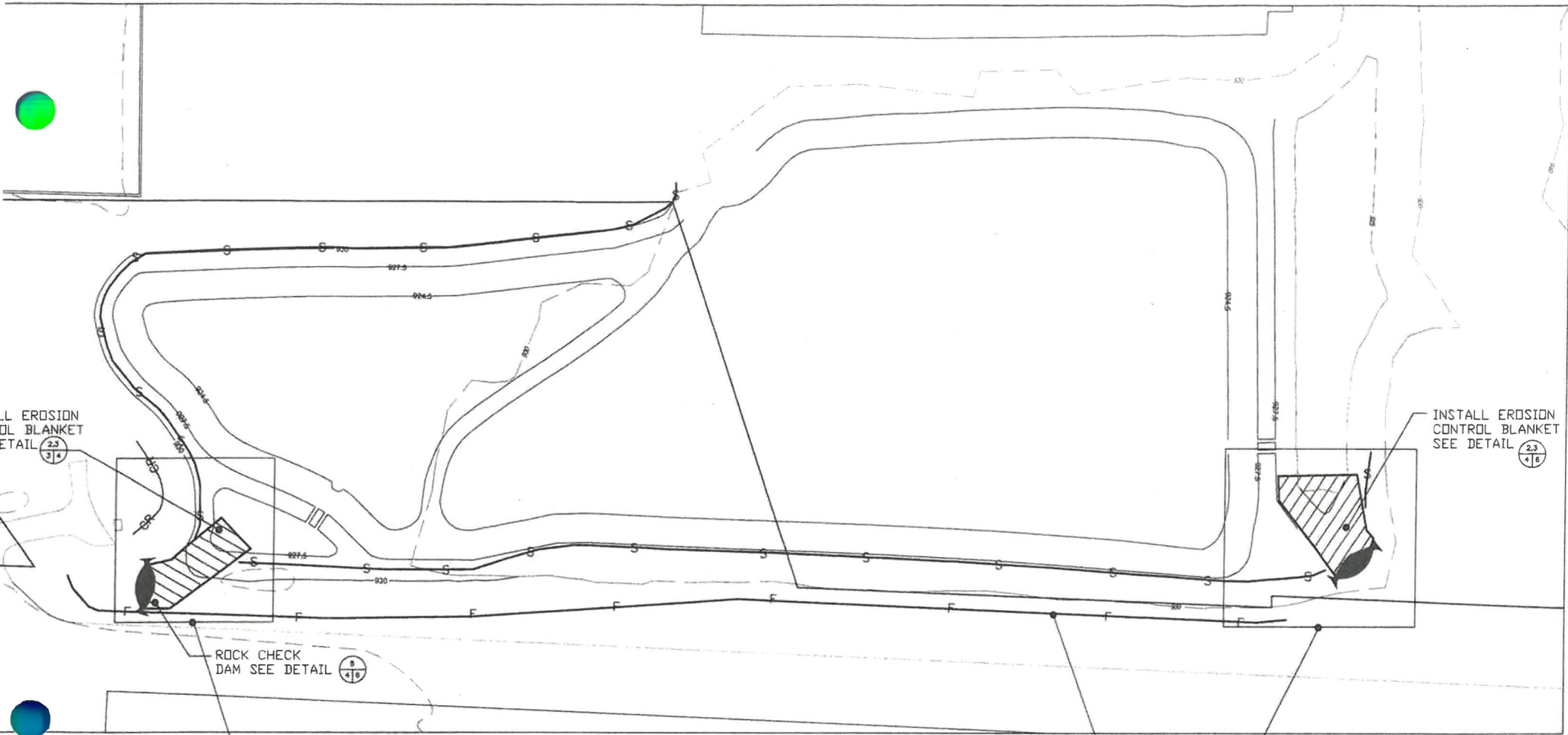
EROSION CONTROL PLAN VIEW SCALE: 1" = 10'
