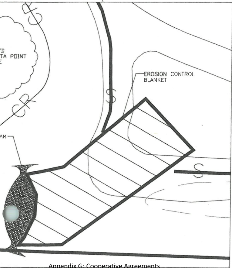
Appendix G: Cooperative Agreements EROSION CONTROL BLANKET INSET SCALE: 1" = 10'
