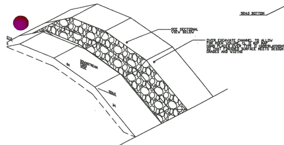
4 OVERFLOW SWALE DETAIL 3/8 NO SCALE
