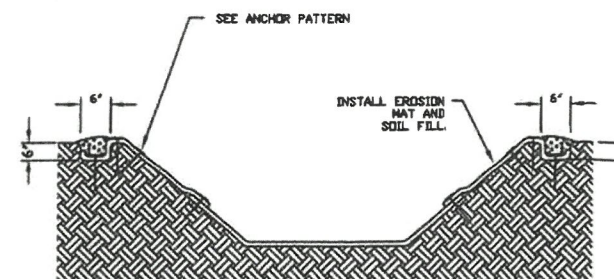
EROSION CONTROL BLANKET DETAIL
