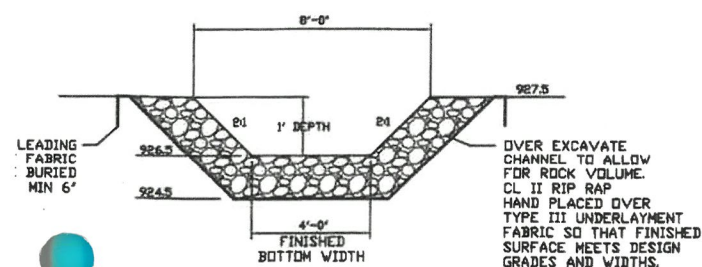
BERM PILOT CHANNEL SECTION
