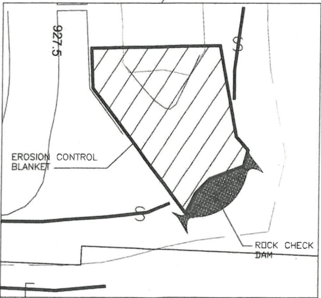
EROSION CONTROL BLANKET INSET SCALE: 1" = 10' - 0'
