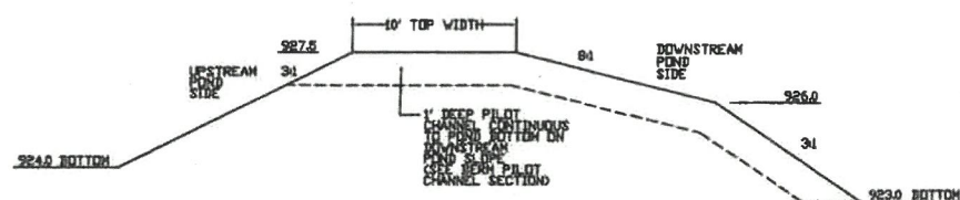
SECTION C C'
