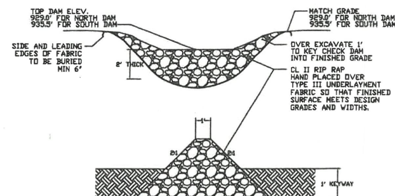
ROCK CHECK DAM SECTION
