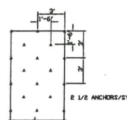
EROSION CONTROL BLANKET ANCHOR PATTERN
