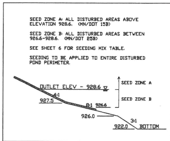
POND EDGE SEEDING PLAN SECTIONAL VIEW NOT TO SCALE
