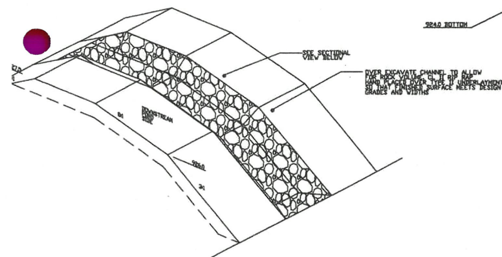
4 OVERFLOW SWALE DETAIL
