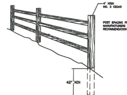
7 TYPICAL CEDAR SPLIT RAIL FENCE DETAIL
