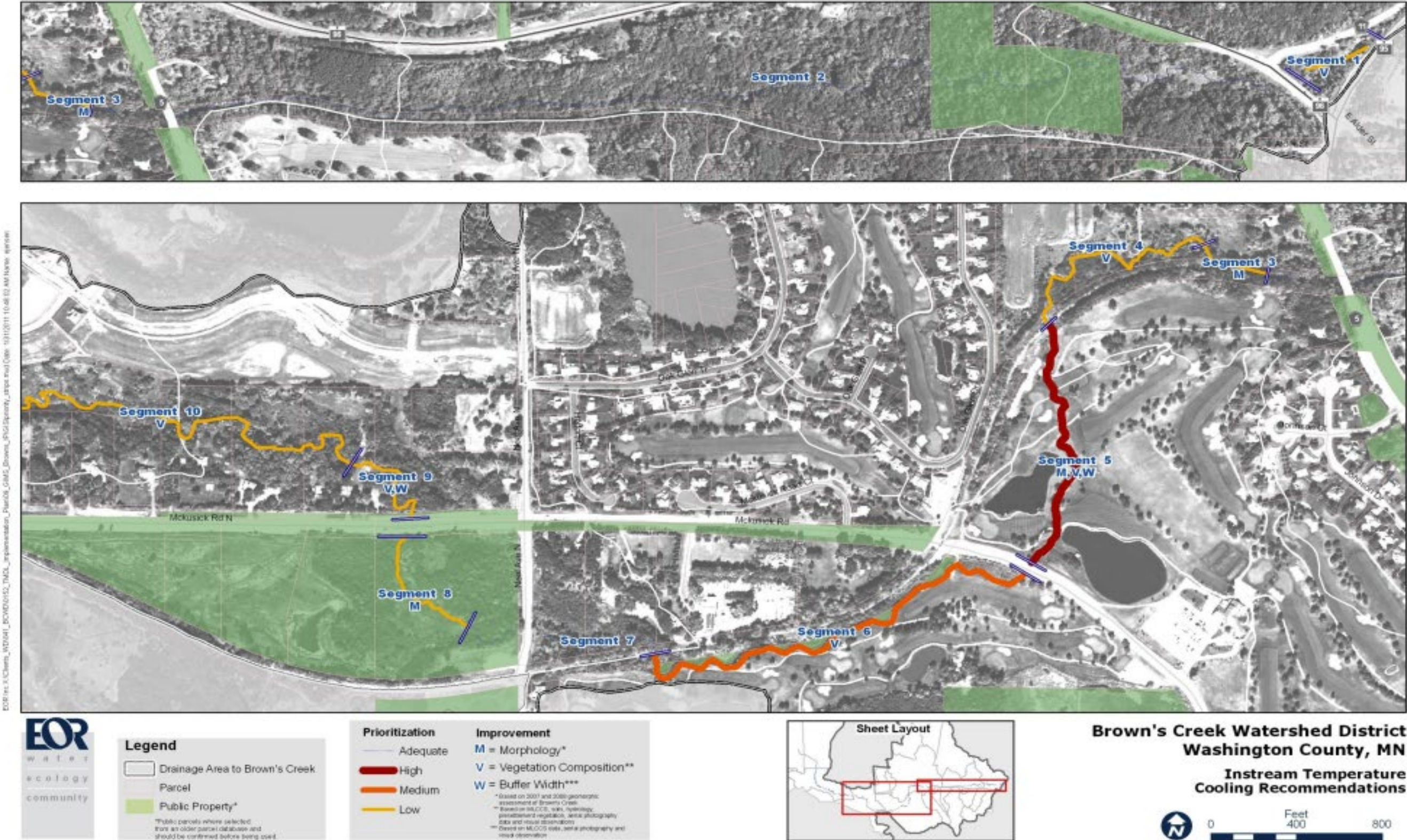
Figure 4. Stream Geomorphology and Thermal Buffer Improvements 2012 (Page 1)
